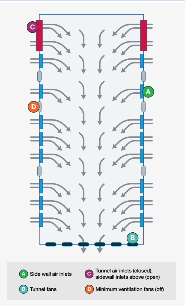
Figure 106 Typical air movement during transitional ventilation.
