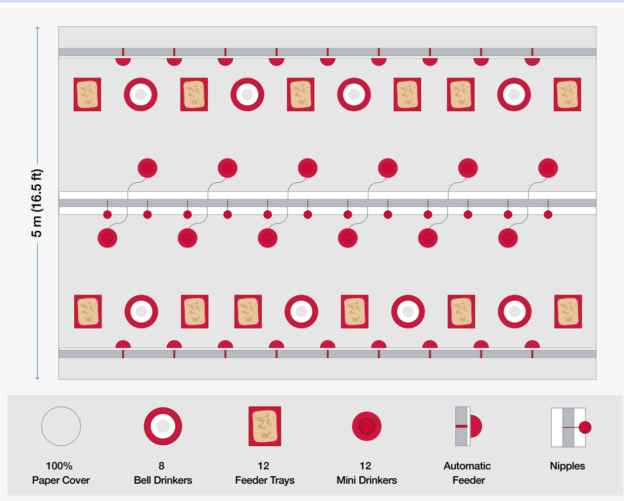
Figure 13 Typical whole-house brooding layout for 1,000 chicks.
