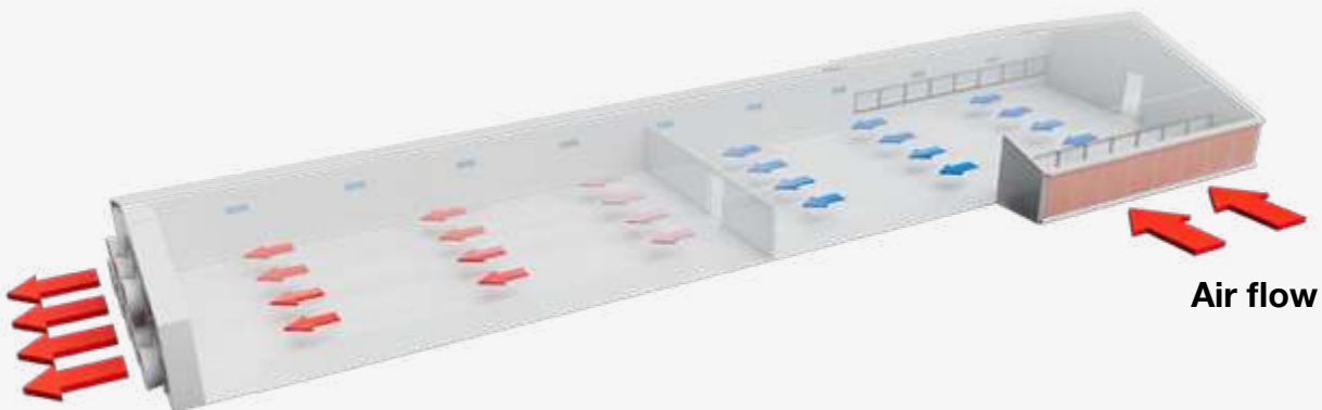
Figure 108 Air flow in a tunnel ventilated house.
