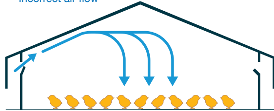
Example 2: Incorrect air flow
