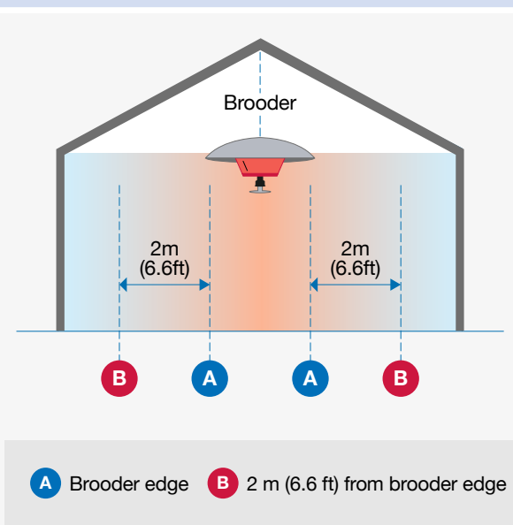
Figure 16 Spot brooding temperature gradients.
