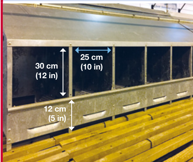
Figure 52 Nest box entrance dimensions.
