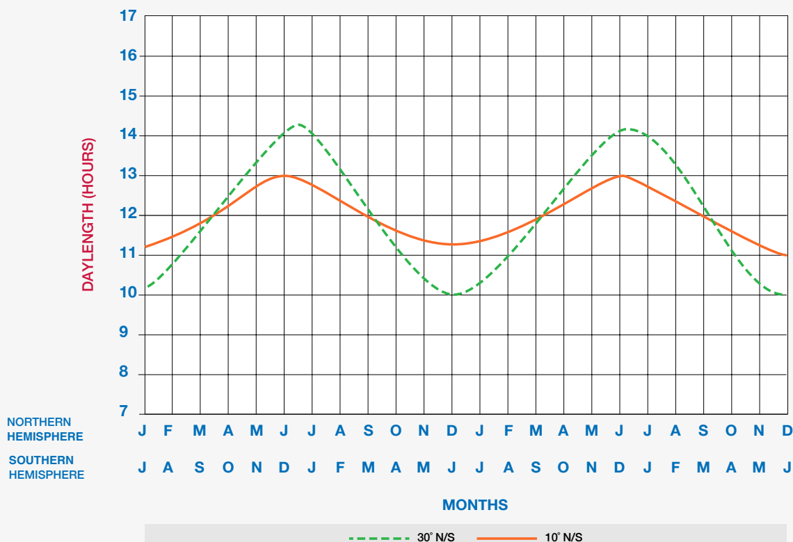
Figure 116 Natural daylengths at latitude 10° or 30° north or south.
